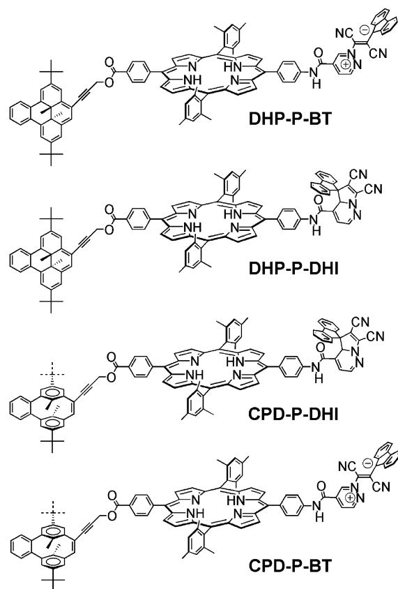
Figure 1. The four isomeric forms of triad 1 .
