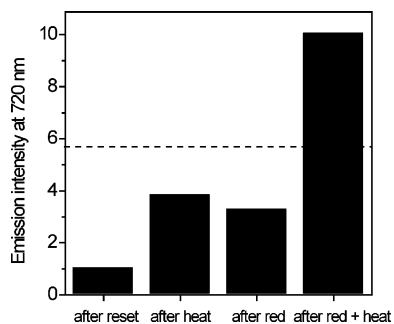
Figure 5. Performance of triad 1 as an AND gate. The bar graph shows the experimental porphyrin emission intensity following the listed inputs. The conditions for the inputs are described in the text. The dashed line represents a hypothetical threshold for readout purposes.
