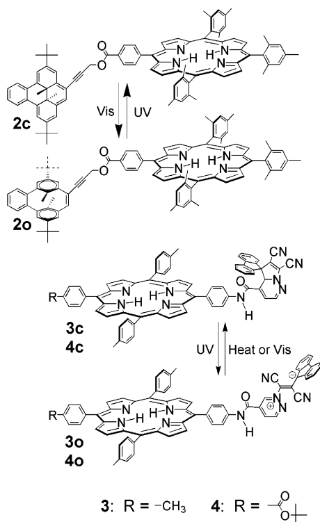
Figure 2. Structures of model compounds 2–4 and their isomeric forms.
