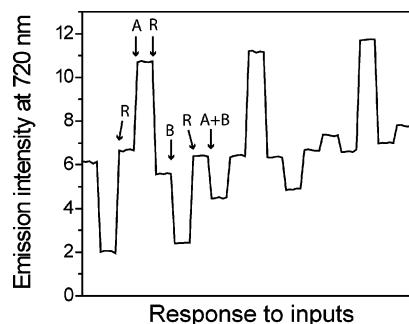
Figure 8. Cycling of the INHIBIT gate. The gate readout with associated random noise is shown following each input (vertical line). A: input A, red light (590 nm < \lambda < 900 nm, 33 mW/cm 2 , 300 s). B: input B, UV light (366 nm, 1.5 mW/cm 2 , 40 s). R: reset (366 nm light, 1.5 mW/cm 2 for 40 s followed by 254 nm light, 700 \mu W/cm 2 , for 5 s, and heat, 55 °C for 30 min).
