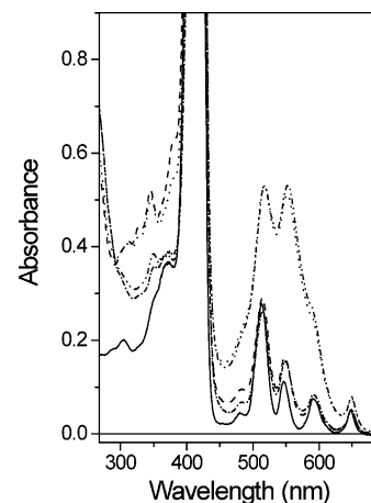
Figure 3. Absorption spectra in 2-methyltetrahydrofuran of pure or highly enriched solutions of 5,15-bis(4-methoxycarbonylphenyl)-10,20-bis(2,4,6-trimethylphenyl)porphyrin (—), CPD-P-DHI (---), DHP-P-DHI (---), CPD-P-BT (---), and DHP-P-BT (---). In some cases, the spectra represent photostationary states, as explained in the text.
