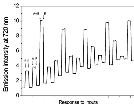
Figure 6. Cycling of the AND gate. The gate readout with associated random noise is shown following each input (vertical line). A: input A, heat (55 °C for 30 min). B: input B, red light (590 nm < \lambda < 900 nm, 33 mW/cm 2 , 300 s). R: reset (366 nm light, 1.5 mW/cm 2 for 40 s followed by 254 nm light, 700 \mu W/cm 2 , for 5 s). The cycle was repeated five times.
