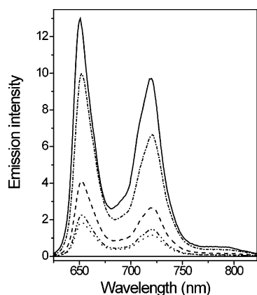
Figure 4. Emission spectra of the different states of triad 1 in 2-methyltetrahydrofuran following excitation at 590 nm: model porphyrin (—), CPD-P-DHI (---), DHP-P-DHI (····), CPD-P-BT (-·-·-), and DHP-P-BT (···)
