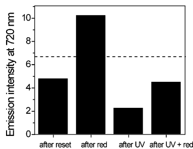
Figure 7. Performance of triad 1 as an INHIBIT gate. The bar graph shows the experimental porphyrin emission intensity following the listed inputs. The conditions for the inputs are described in the text. The dashed line represents a hypothetical threshold for readout purposes.
